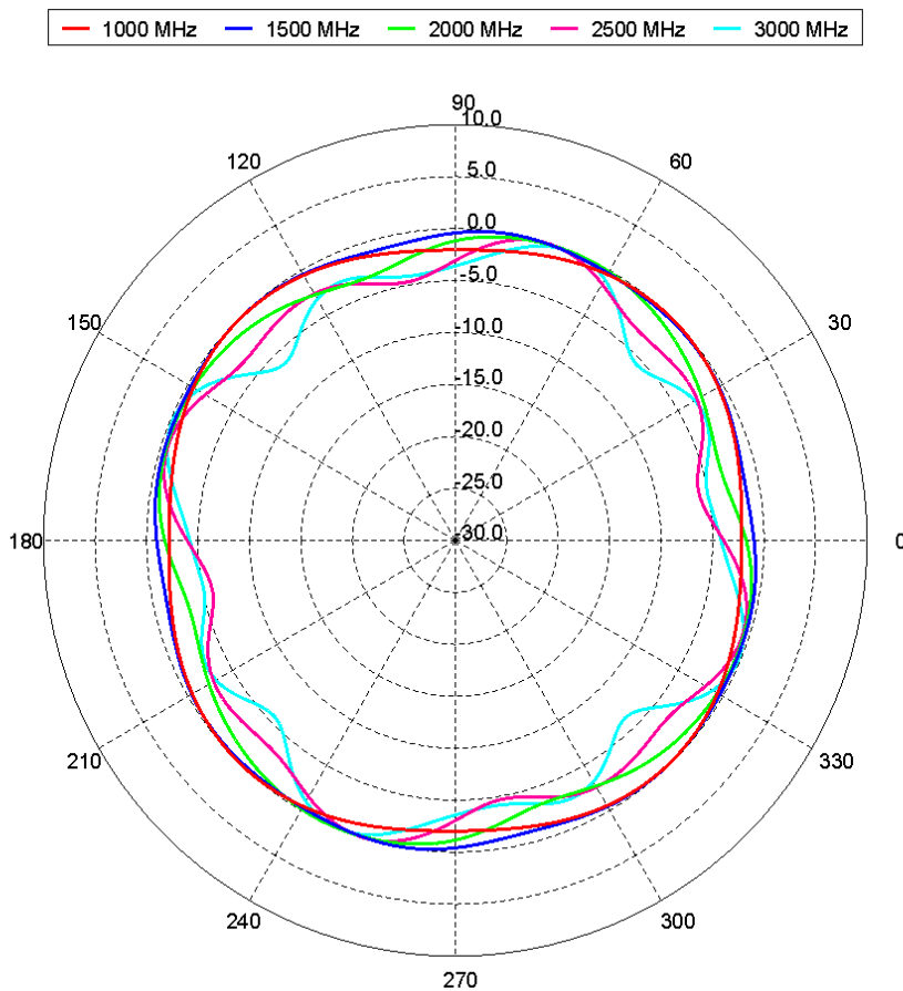
Normalised Azimuth (E-Plane) Pattern for Band B
